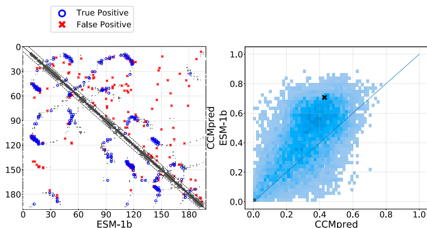
Fig. 5. Residue-residue contacts (linear projections). (Left) Top-L predictions for fold level held-out example d1n3ya_ with vWA-like fold. True positives in blue, false positives in red, superimposed on ground truth contact map in gray. ESM-1b Transformer projections below the diagonal, CCMpred predictions above the diagonal. (Right) Precision distribution (top-L long-range) comparing ESM-1b projections with CCMpred across all domains in the five test partitions with structural holdout at the fold level. Visualized domain marked by \times .
